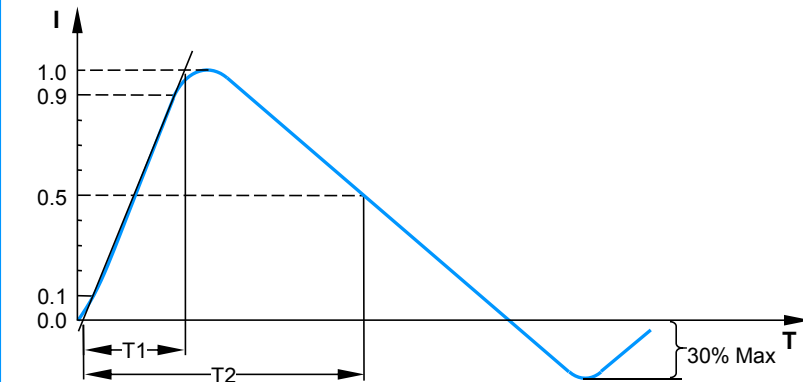
Wave shape "Short Circuit" (Current I_{sc} )
